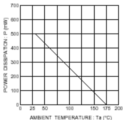
Fig.2 Derating curve
